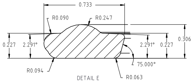
DETAIL E SCALE 2 : 1
