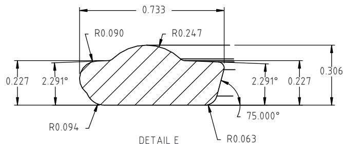
DETAIL E SCALE 2 : 1
