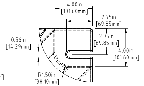
DETAIL A SCALE 1:6
